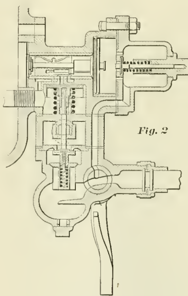
A REINFORCED BRAKE.
